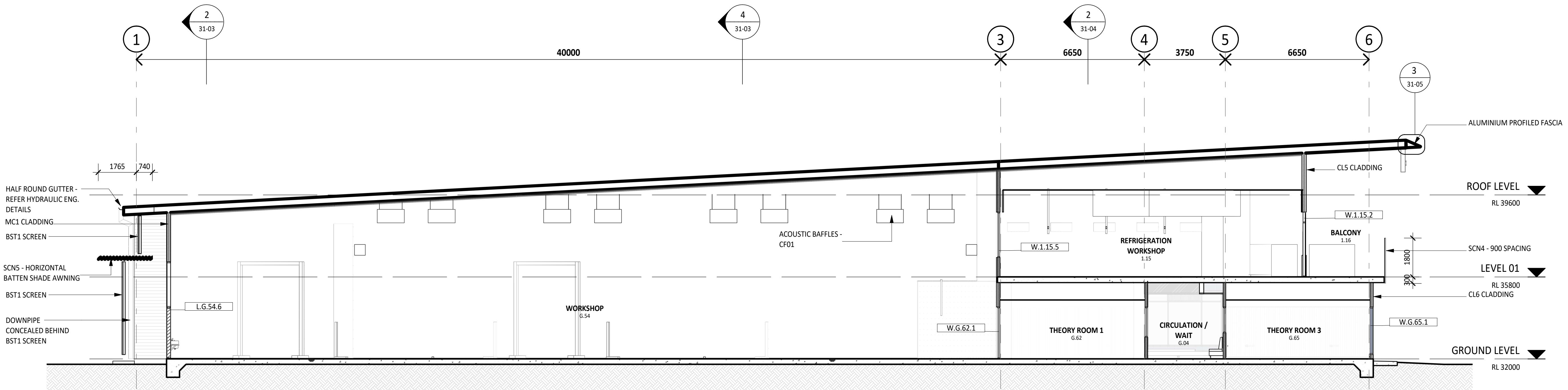
1 BUILDING SECTION - 4 21-01 1 : 100
